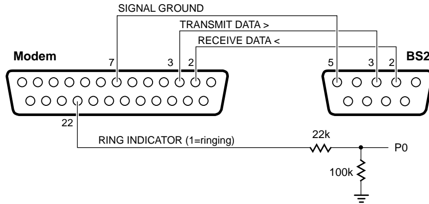
Figure 1. Modem-to-BS2 Hookup.
